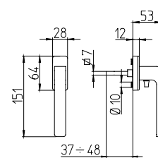
1682/DK-SIC martellina dk drehkipp system
